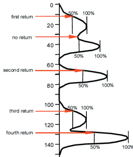
Fig. 2. Lidar multiple return signal
